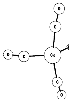
Figure 5. CC conformation of \text{HCo}(\text{CO})_3 , ^1A'' .
