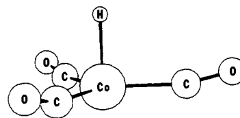
Figure 3. HV conformation of \text{HCo}(\text{CO})_3 , ^1A_1 .
