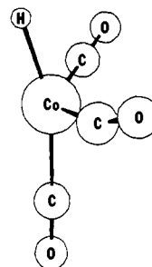
Figure 4. HC conformation of \text{HCo}(\text{CO})_3 , ^1A' .
